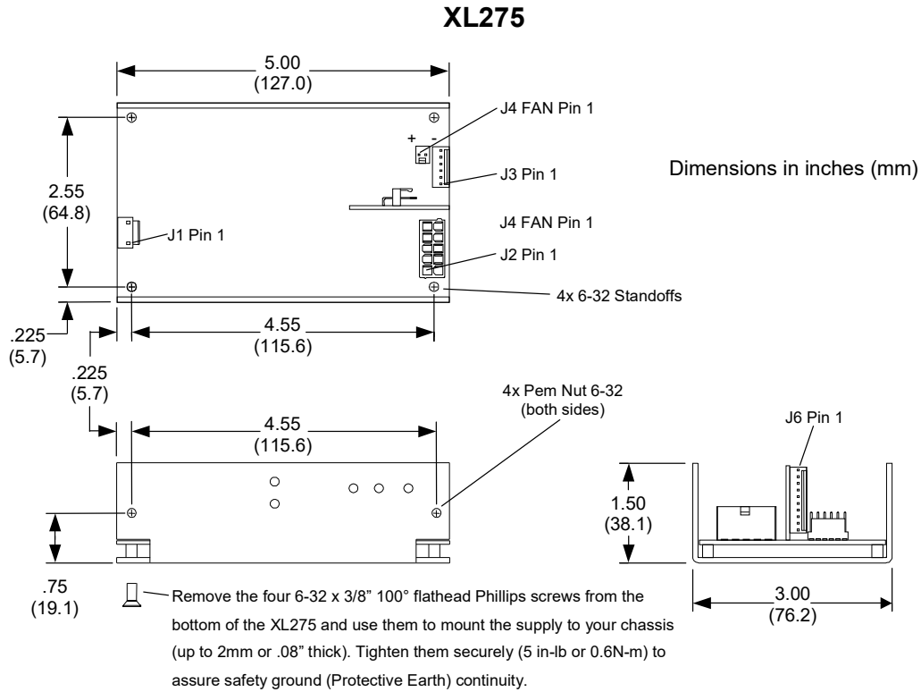
Figure 4-1 XL275 Dimensions
