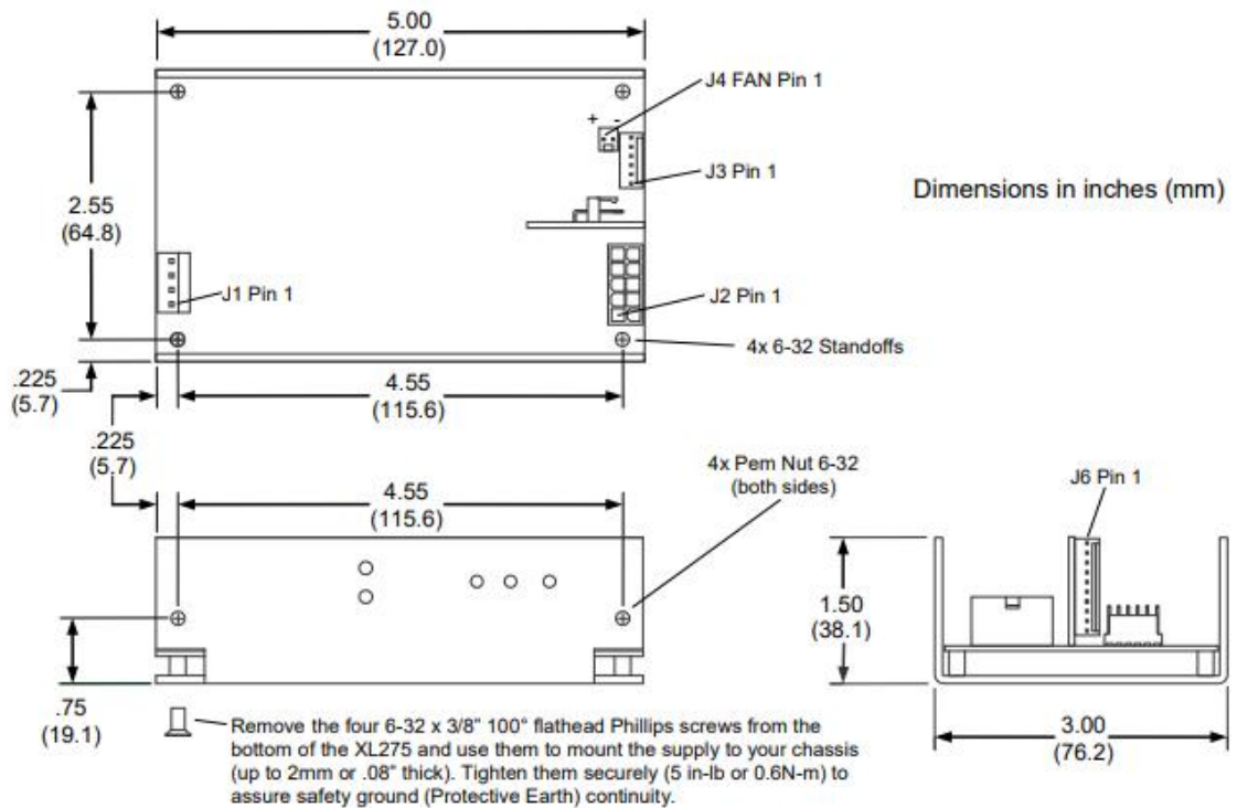
Figure 4-2 XL275-DC Dimensions
