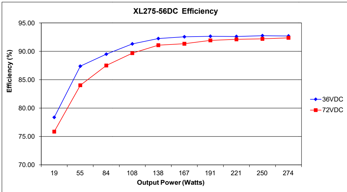
Figure 3-5 XL275-56DC Efficiency
