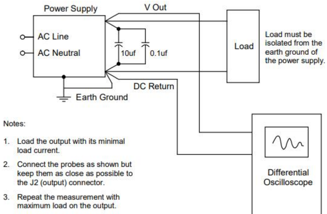
Figure 3-7 Ripple Noise Measurement Setup
