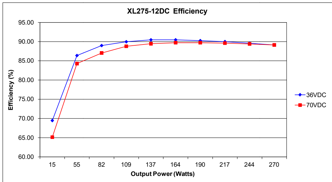
Figure 3-1 XL275-12DC Efficiency
