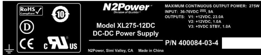
Figure 4-1 Sample XL275-DC Label
